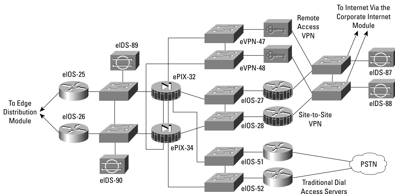
Figure 36 VPN and Remote Access Module: Detail
