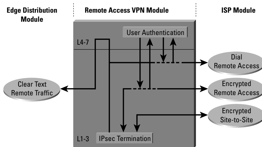
Figure 21 Remote Access VPN Module Traffic Flow
