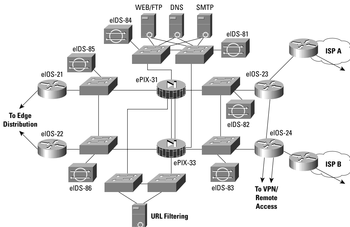
Figure 35 Corporate Internet Module: Detail
