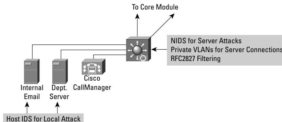
Figure 13 Attack Mitigation Roles for Server Module
