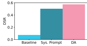
Figure 18: DA's Performance on Software Security Guidance
