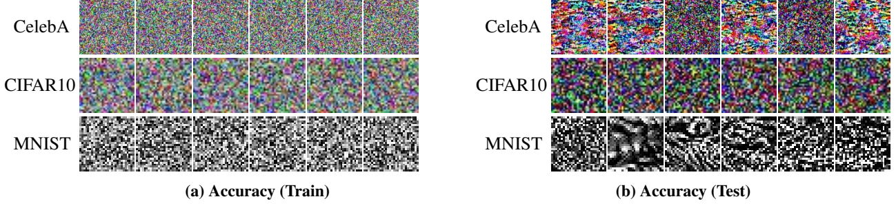
Figure 7: Counterexamples of accuracy-based metrics. The left examples show that using random-like samples can train a well-generalized model, and the right examples demonstrate that random-like samples can be predicted with high confidence.
