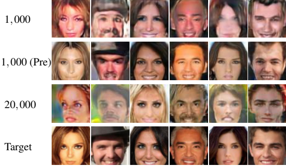
Figure 3: Visualization of PLGMI on different target models.
