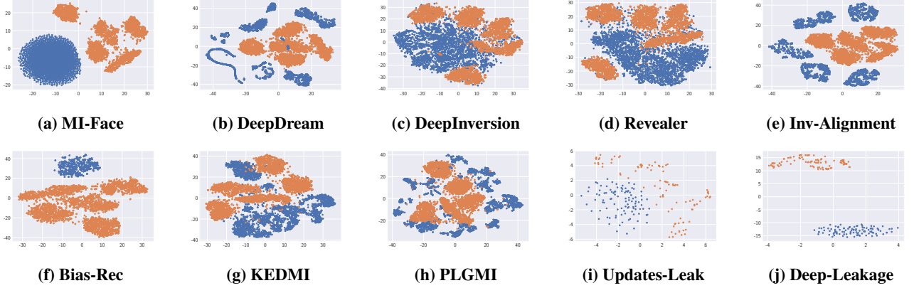
Figure 10: t-SNE visualization of reconstructions and corresponding target datasets for MNIST.
