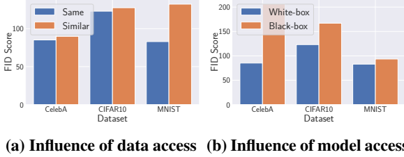
Figure 4: Influence of auxiliary information for PLGMI. Experimental results for other attacks can be found in Figure 14.
