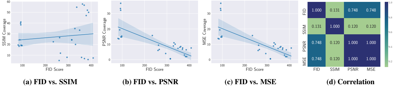
Figure 12: Relationship between coverages calculated with different sample-level metrics and the dataset-level metric for CelebA, we plot the correlation heatmap using the absolute value of correlation between different metrics.
