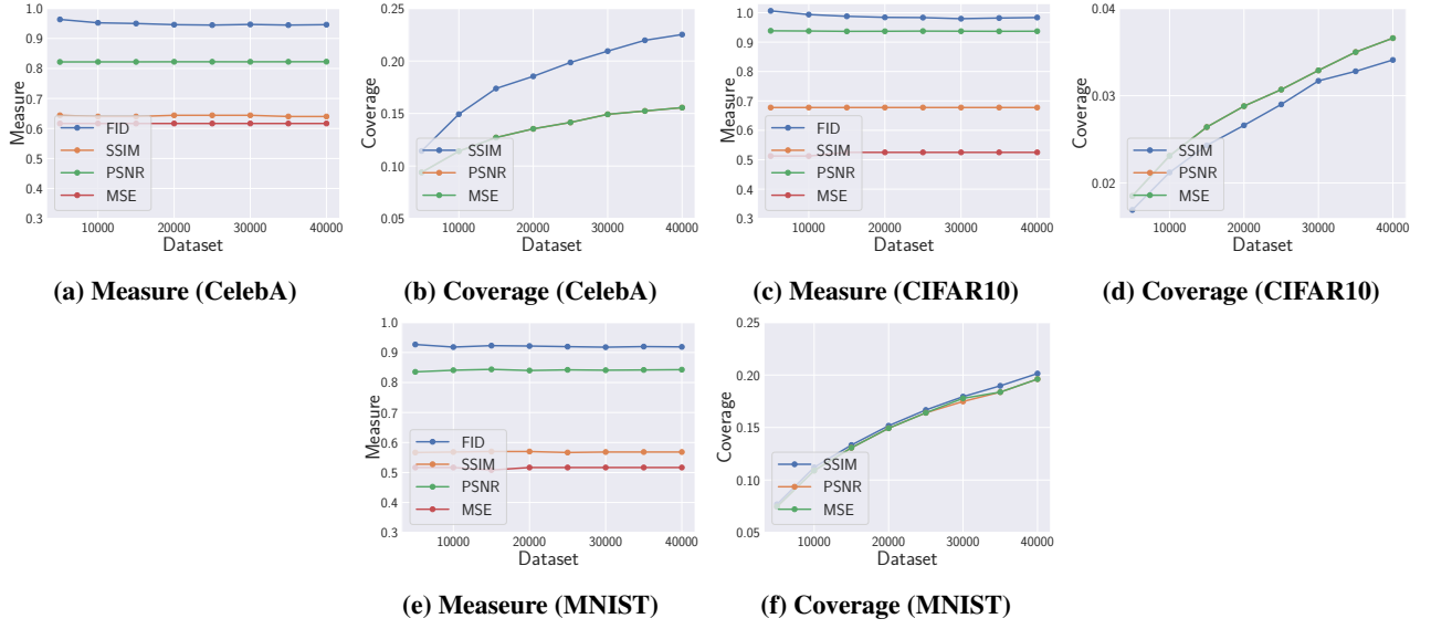
Figure 13: Influence of reconstruction quantity. For ease of presentation, values are normalized to fit the same y-axis.
