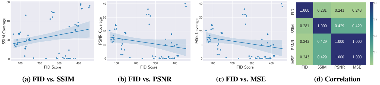
Figure 11: Relationship between coverages calculated with different sample-level metrics and the dataset-level metric for CIFAR-10 and MNIST, we plot the correlation heatmap using the absolute value of correlation between different metrics.
