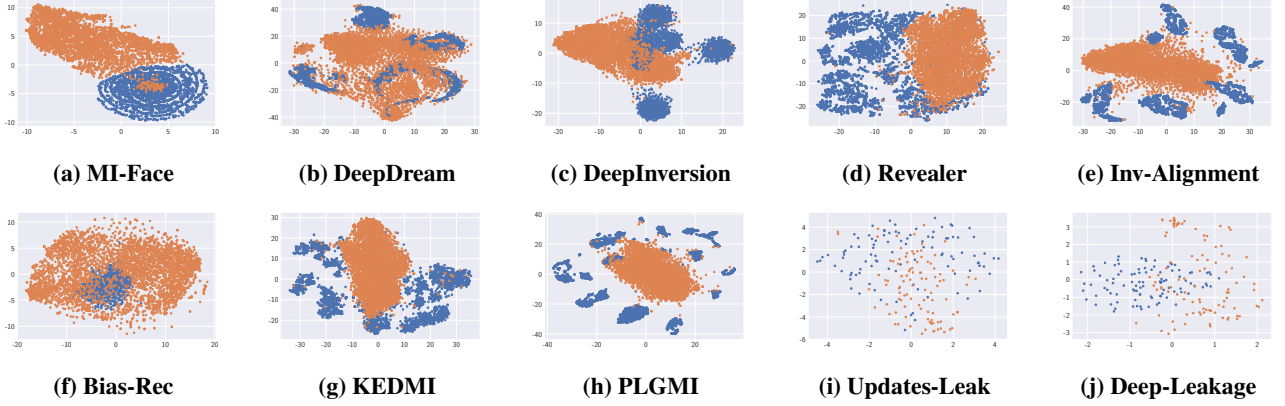
Figure 9: t-SNE visualization of reconstructions and corresponding target datasets for CIFAR10.
