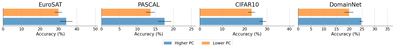
Figure 6: Comparison of attacker model accuracy using synthetic images generated from prompts with higher and lower prompt consistency across four datasets.
