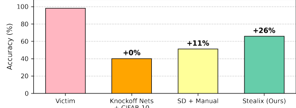
Figure 1: Impact of query datasets on stealing a satellite image classifier: performance drops occur with dissimilar datasets (Knockoff Nets + CIFAR-10) and challenging prompt design (SD + manual). Stealix mitigates these issues by leveraging victim-aware automatic prompt tuning.
