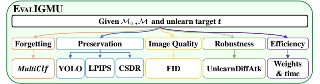
Figure 6: The overview and implementation of the proposed evaluation framework, EVALIGMU, for machine unlearning for IGM. It considers five aspects: Forget , Preserve , Image Quality , Robustness , and Efficiency . Some quantitative metrics are listed for each of them as one implementation of EVALIGMU.
